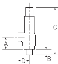
Male screwed
